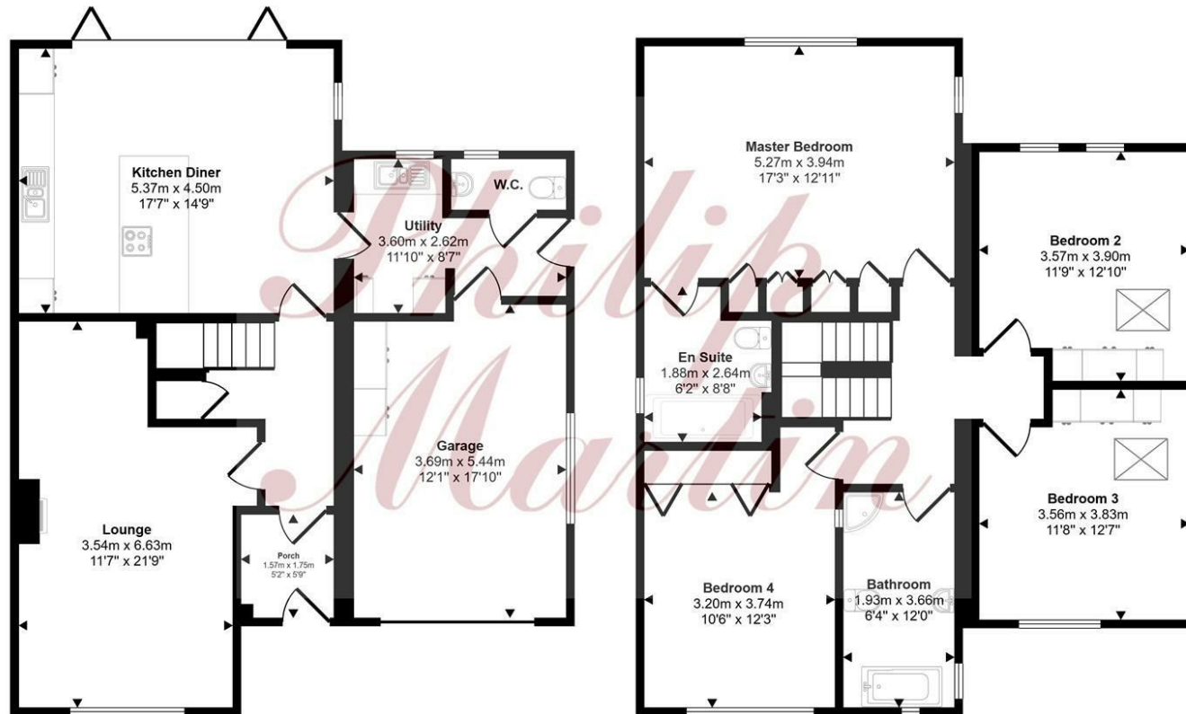
Ground Floor Approx 89 sq m / 954 sq ft
